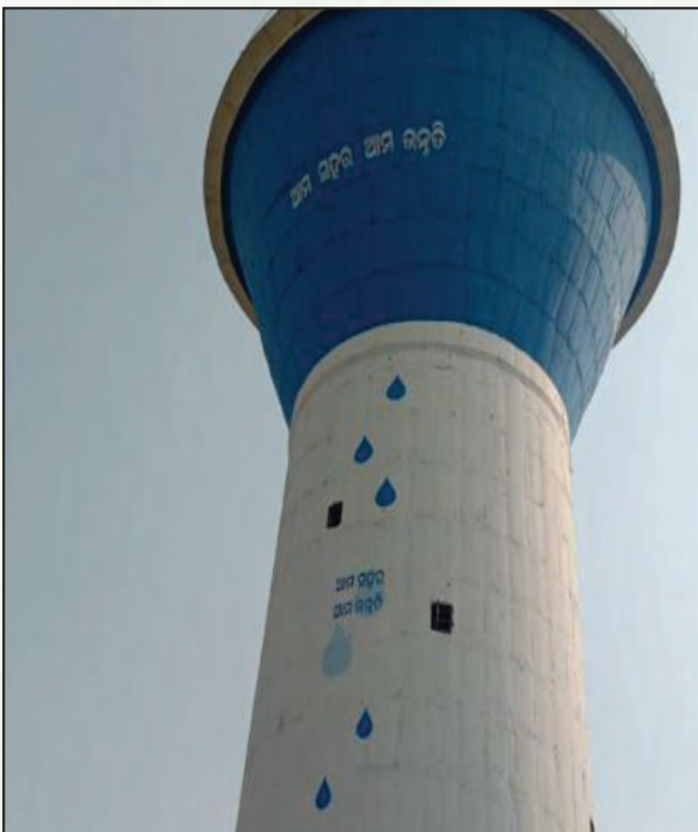
Special repair of 4.54 Lakh litre capacity ESR at Dhabalagiri including replacement of valves and interconnection work.
